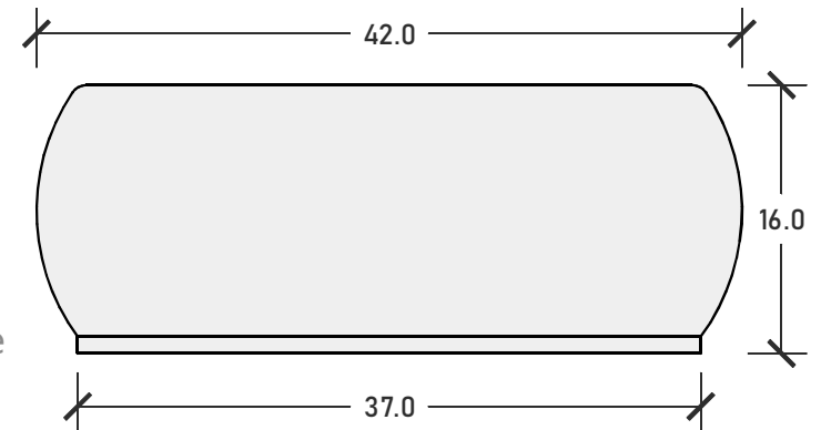
Fianco | Side
