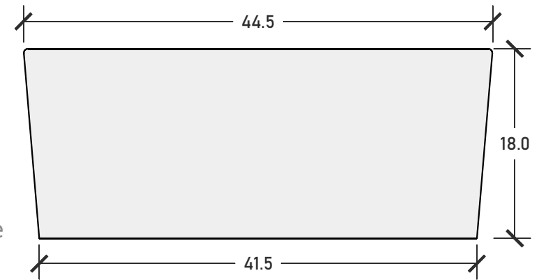
Fianco | Side
