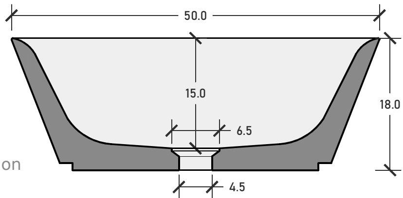
Fianco | Side
