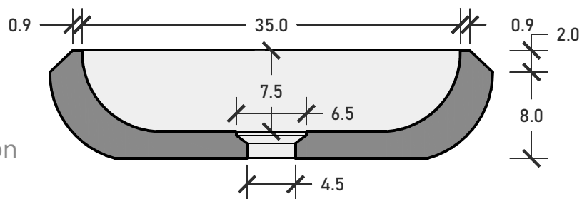
Fianco | Side
